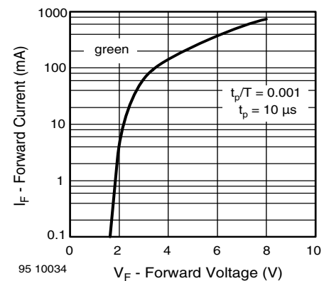
Fig. 18 - Forward Current vs. Forward Voltage
