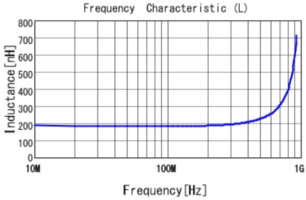
LQW2BASR18J00 L
