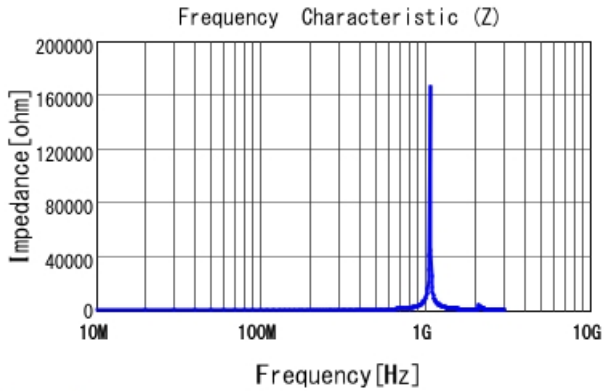
LQW2BASR18J00 |Z|
