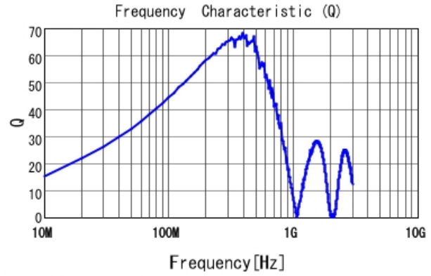
LQW2BASR18J00 Q
