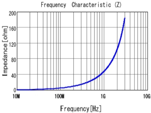
■ LQP03TN7N5J02 |Z|
