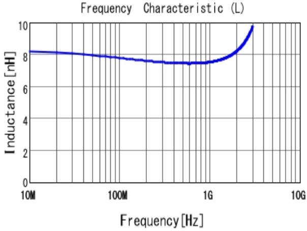
■ LQP03TN7N5J02 L
