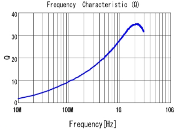
■ LQP03TN7N5J02 Q
