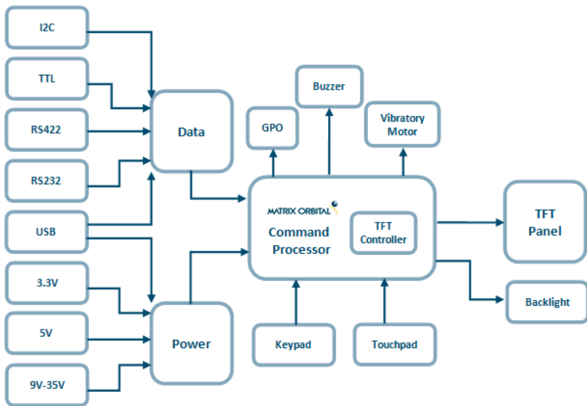
Figure 2: Functional Diagram
