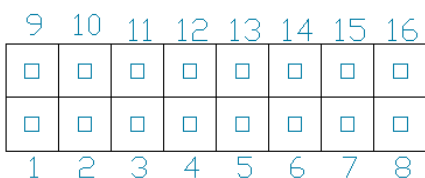
Figure 15: GPO Header
