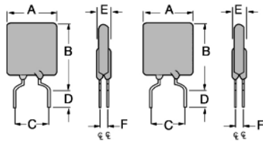
Fig.3 Lead Size : 20AWG Φ 0.81 mm Diameter
