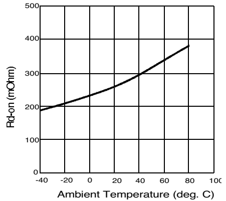
Figure 4. Typical On-Resistance
