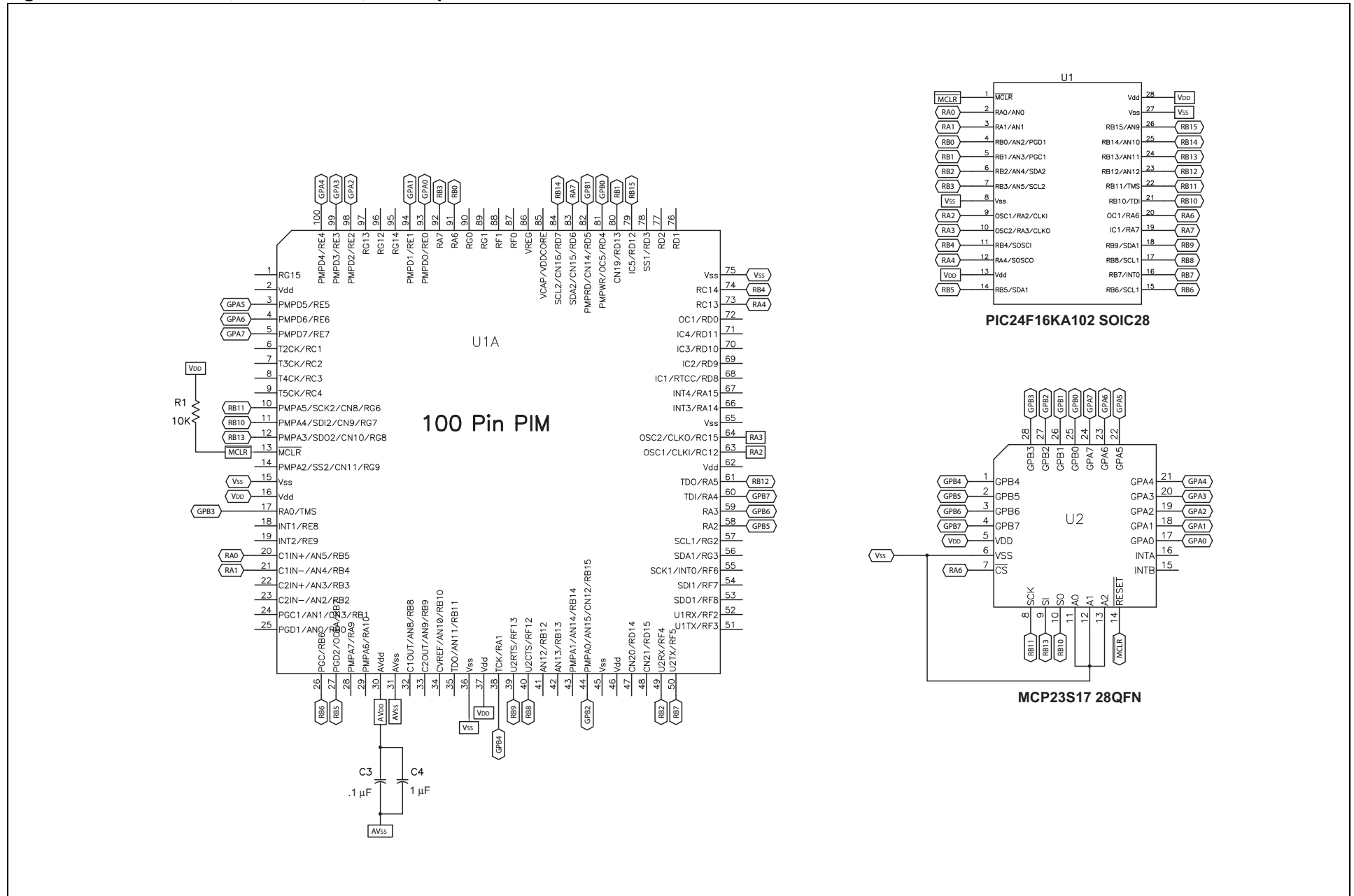
Figure 1: 100-Pin Header, 28-Pin Device, Port Expander Schematic
