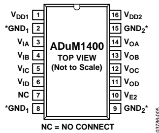
Figure 5. ADuM1400 Pin Configuration
