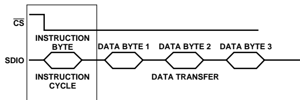
Figure 51. Using SDIO as a Read/Write Transfer
