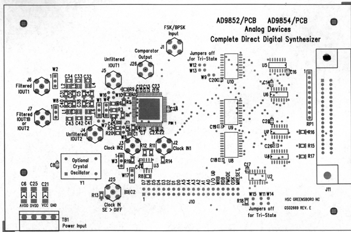
Figure 67. Assembly Drawing
