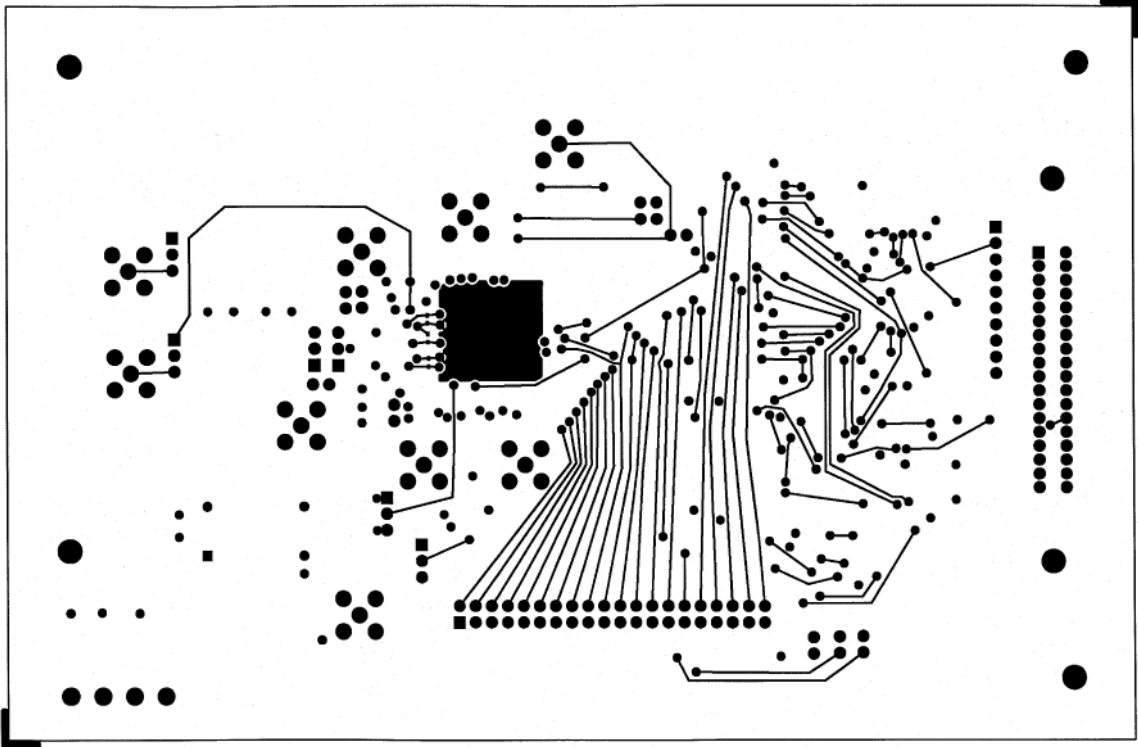
Figure 71. Bottom Routing Layer, Layer 4
