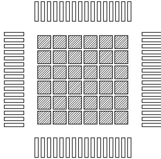
Figure 64. Proposed Solder Placement
