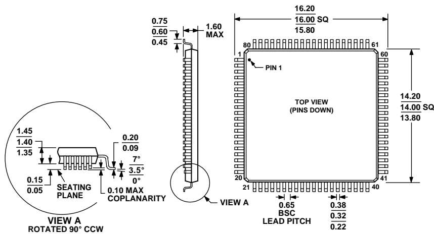
COMPLIANT TO JEDEC STANDARDS MS-026-BEC Figure 73. 80-Lead Low Profile Quad Flat Package [LQFP] (ST-80-2) Dimensions shown in millimeters
