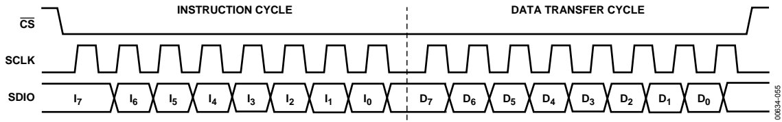
Figure 55. Serial Port Write Timing Clock Stall Low
