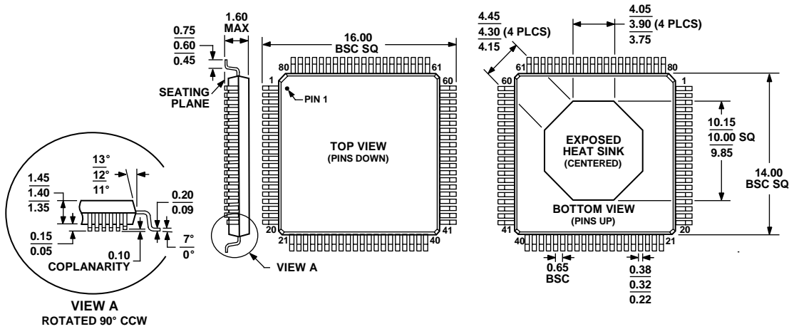
COMPLIANT TO JEDEC STANDARDS MS-026-BEC-HD Figure 72. 80-Lead Low Profile Quad Flat Package, Edquad [LQFP_ED] (SQ-80-2) Dimensions shown in millimeters
