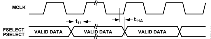
Figure 4. Control Timing
