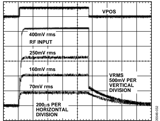
Figure 32. Output Response to Gating on Power Supply for Various RF Input Levels, Supply 3 V, Modulation Frequency 900 MHz, 0.01 \mu F Filter Capacitor
