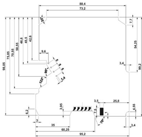
Dimensional drawing of the ME MAX U-U1 printed circuit board, for printed circuit terminal block connection (MKDSO), view: component side
