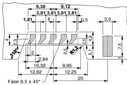
Dimensional drawing of the ME MAX U-U1 printed circuit board, for printed circuit terminal block connection (MKDSO), view: component side
