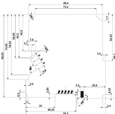
Dimensional drawing of the ME MAX U-U1 printed circuit board for plug connection (MSTBO), view: component side
