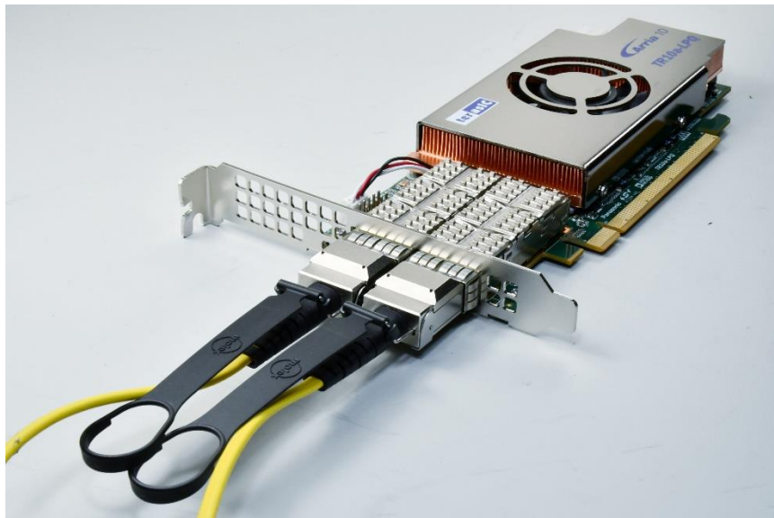
Figure 7-3 One QSFP+ Cables Installed
