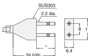
Using the E32-D61
