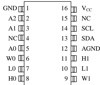
DS1807S 16-Pin SOIC (150-mil) See mech. Drawings Section
