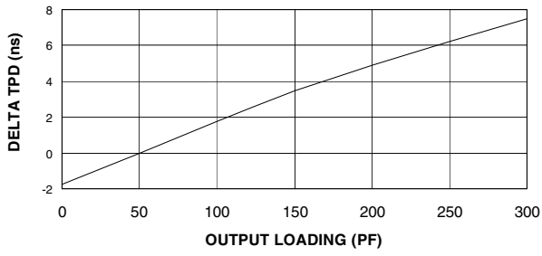
ATF22V10C DELTA T_{PD} vs. OUTPUT LOADING
