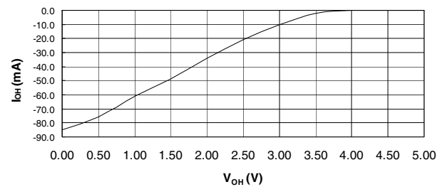
ATF22V10CZ/CQZ OUTPUT SOURCE CURRENT vs. OUTPUT VOLTAGE ( V_{CC} = 5\text{V} , T_A = 25^\circ\text{C} )
