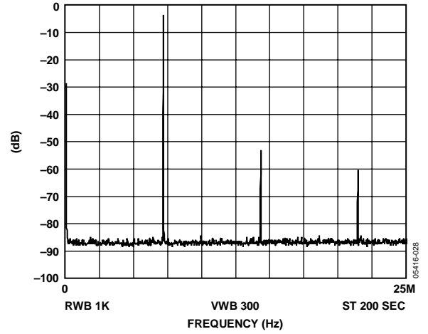
Figure 28. f_{MCLK} = 50 \text{ MHz} , f_{OUT} = 7.143 \text{ MHz} = f_{MCLK}/7 , Frequency Word = 2492492
