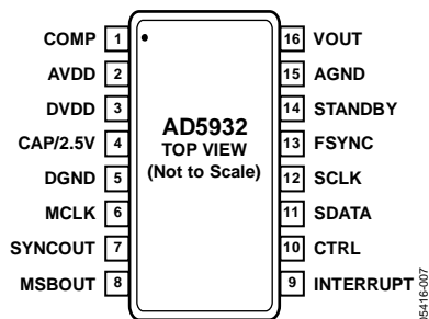
Figure 7. Pin Configuration
