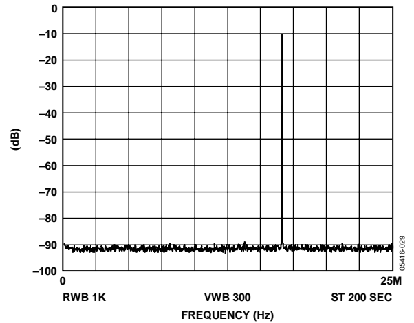
Figure 29. f_{MCLK} = 50 \text{ MHz} , f_{OUT} = 16.667 \text{ MHz} = f_{MCLK}/3 , Frequency Word = 5555555
