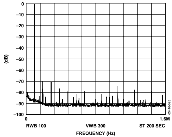
Figure 25. f_{MCLK} = 50 \text{ MHz} , f_{OUT} = 120 \text{ kHz} , Frequency Word = 009D496
