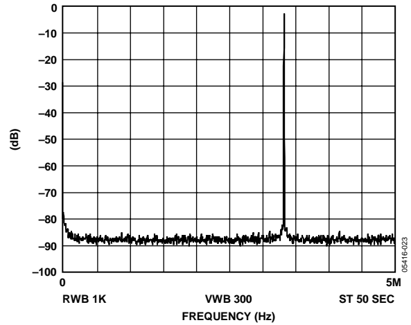
Figure 23. f_{MCLK} = 10 \text{ MHz} , f_{OUT} = 3.33 \text{ MHz} = f_{MCLK}/3 , Frequency Word = 5555555
