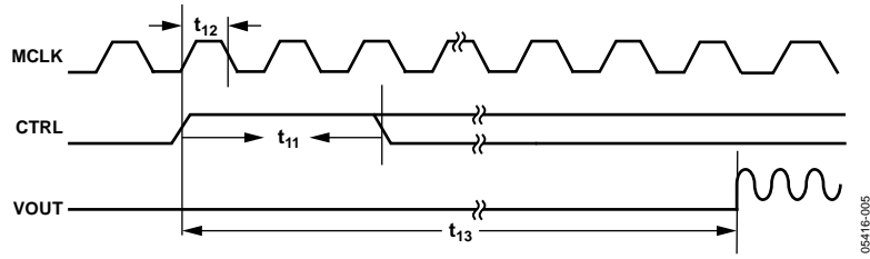
Figure 5. CTRL Timing
