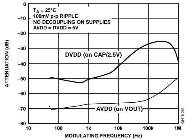
Figure 19. PSRR
