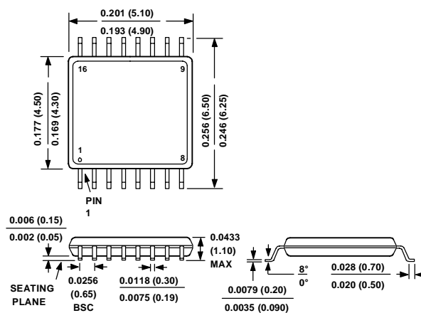
Figure 40. 16-Lead Thin Shrink Small Outline Package (TSSOP) (RU-16)
