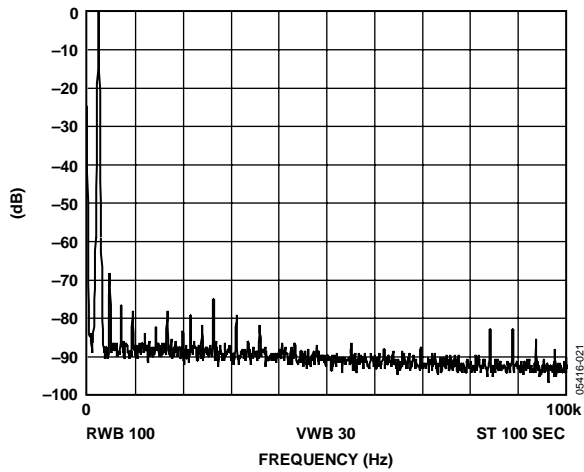
Figure 21. f_{MCLK} = 10 \text{ MHz} , f_{OUT} = 2.4 \text{ kHz} , Frequency Word = 000FBA9
