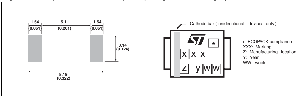
Figure 13. Footprint dimensions mm (inches) Figure 14. Marking layout (1)
