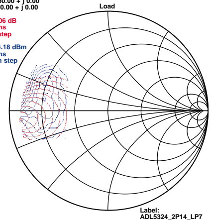
Figure 36. Load-Pull Contours, 2140 MHz
