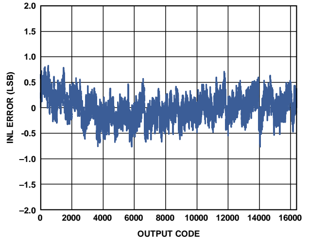
Figure 22. INL Error with f_{IN} = 9.7 MHz
