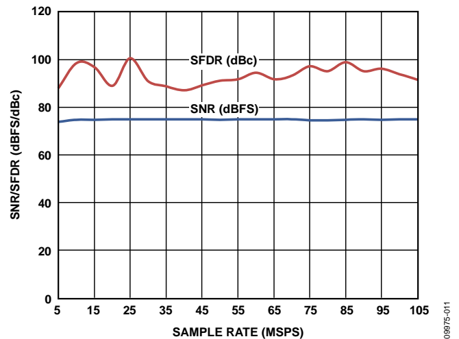
Figure 32. SNR/SFDR vs. Sample Rate with AIN = 70.1 MHz
