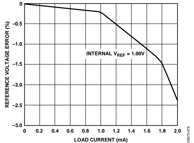
Figure 50. VREF Accuracy vs. Load Current
