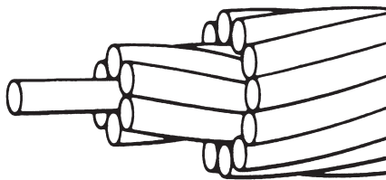
True Concentric and Equilay Stranding
