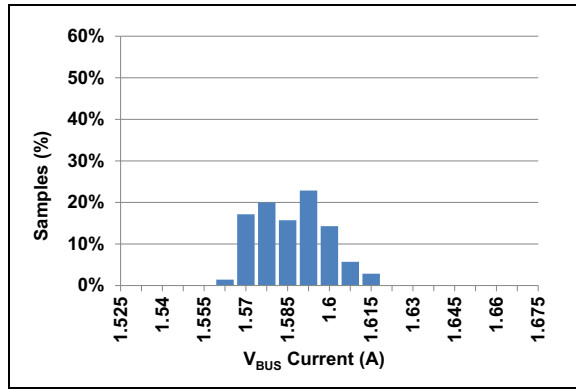
FIGURE 2-17: ILIM5 Trip Current Distribution (1) .
