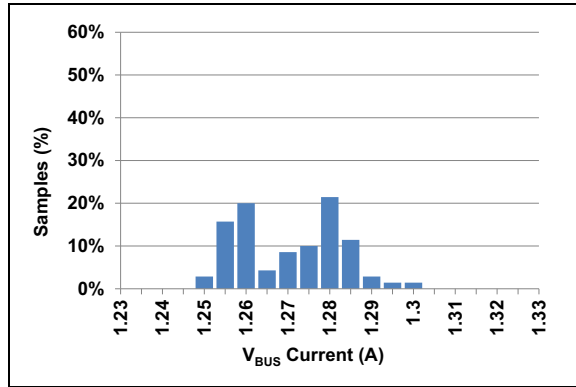
FIGURE 2-16: ILIM4 Trip Current Distribution (1) .
