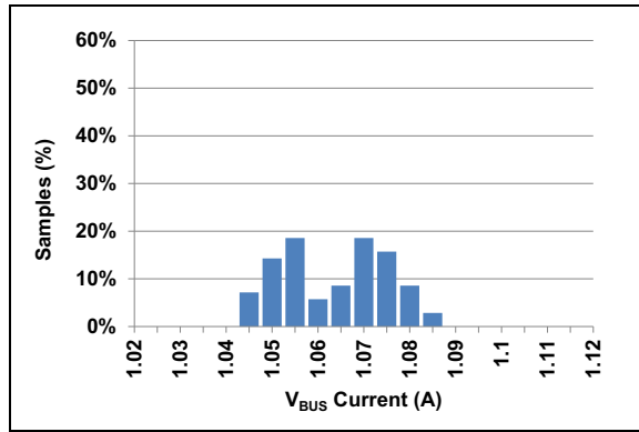
FIGURE 2-15: ILIM3 Trip Current Distribution (1) .
