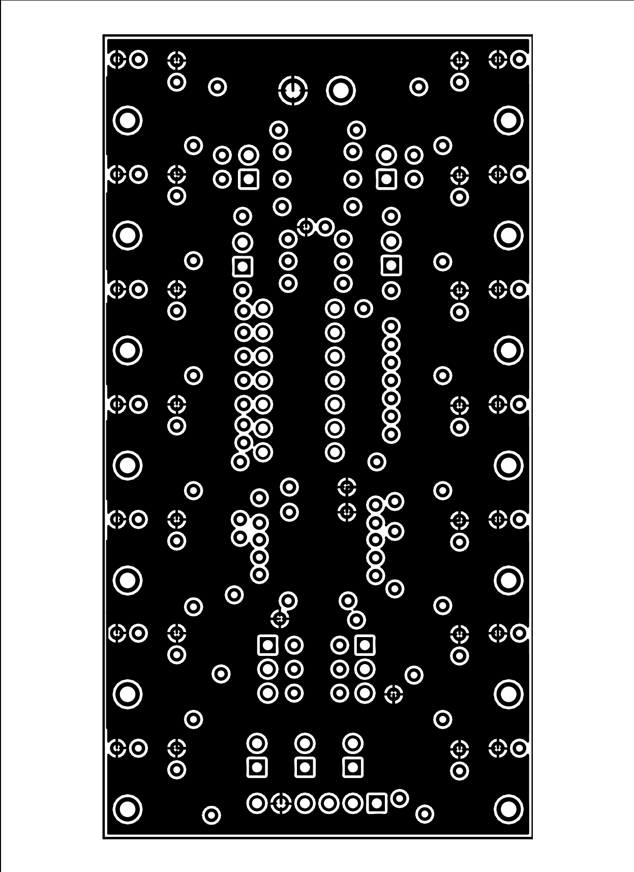
FIGURE A-8: Board Layout – Ground Plane.
