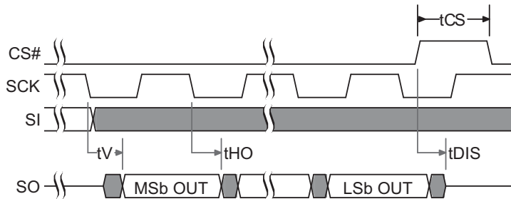
Figure 30. SPI Single Bit Output Timing
