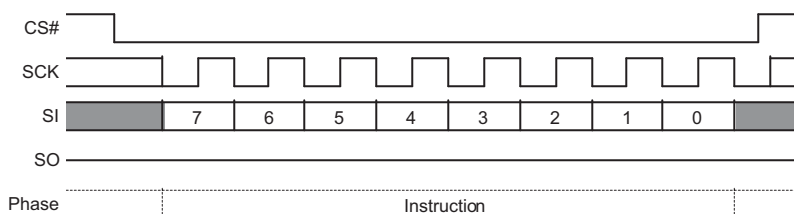
Figure 106. PPB Erase Command Sequence
