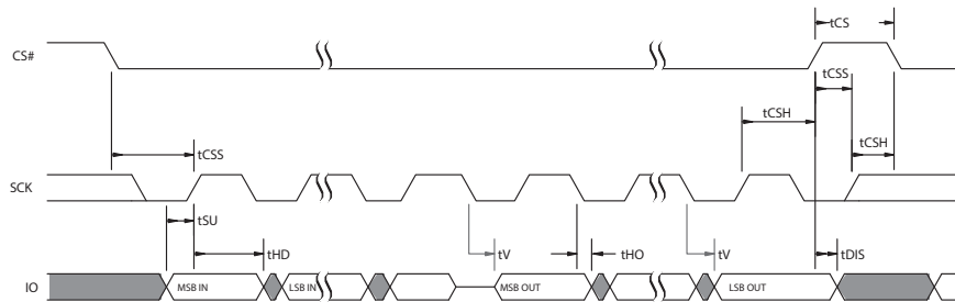
Figure 31. SPI SDR MIO Timing
