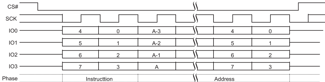
Figure 89. Parameter Sector Erase (P4E 20h or 4P4E 21h) QPI Mode Command Sequence [67]
