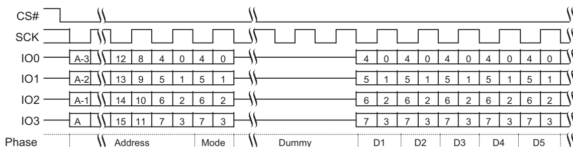
Figure 84. Continuous DDR Quad I/O Read Subsequent Access (EDh or EEh) [60, 61]
