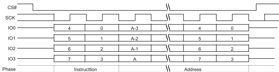
Figure 95. EES QPI Mode Command Sequence [70]
