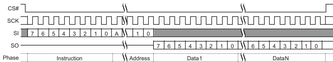
Figure 76. Read Command Sequence (3-Byte Address, 03h or 13h) [51]
