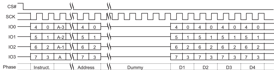
Figure 74. Read Any Register, QPI Mode, Command Sequence [50]
