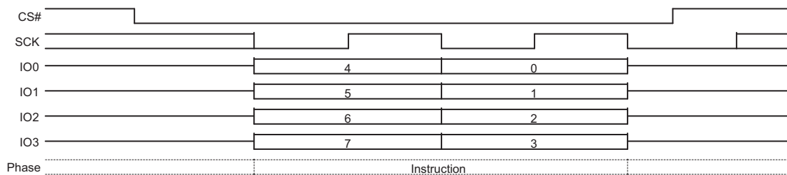
Figure 118. Mode Bit Reset Command Sequence QPI Mode
