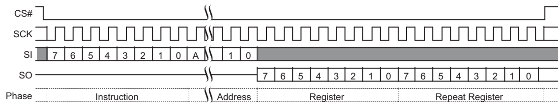
Figure 107. PPBRD Command Sequence [75, 76]
