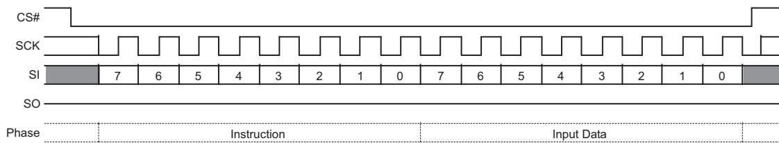
Figure 69. Program NVDLR (PNVDLR) Command Sequence
