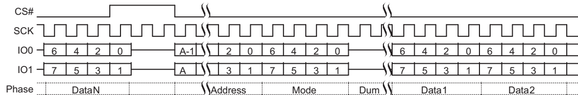
Figure 79. Dual I/O Continuous Read Command Sequence (4-Byte Address [CR2V[7] = 1]) [53, 54]
