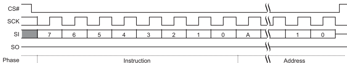
Figure 88. Parameter Sector Erase (P4E 20h or 4P4E 21h) Command Sequence [66]
