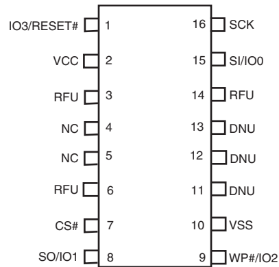
Figure 35. 16-Lead SOIC Package (SO3016), Top View [32]
