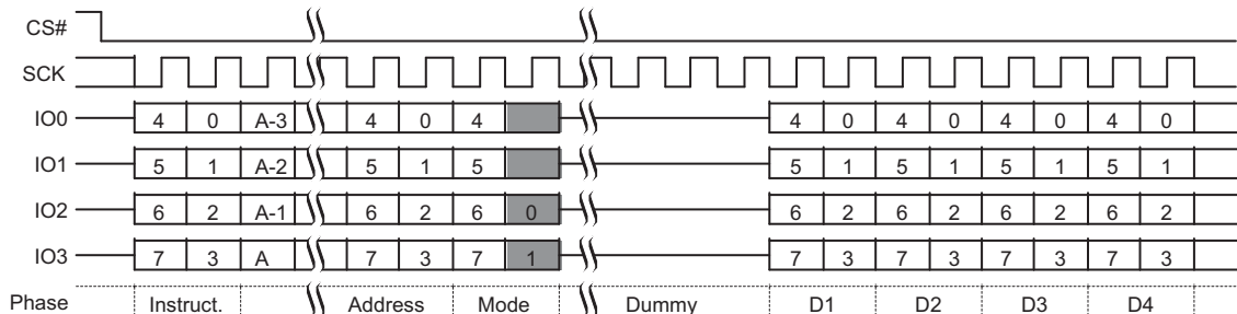
Figure 81. Quad I/O Read Command Sequence (EBh or ECh), QPI Mode [56, 57]
