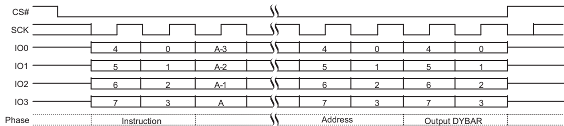
Figure 104. DYBRD QPI Mode Command Sequence [71, 72]
