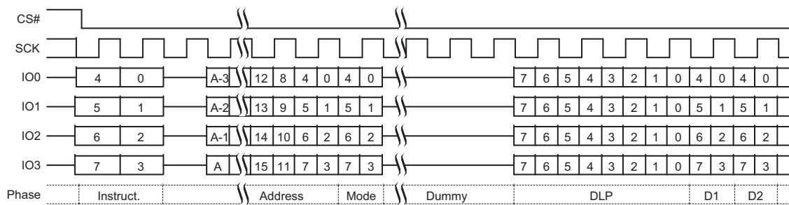
Figure 85. DDR Quad I/O Read Initial Access (EDh or EEh), QPI Mode [62, 63]
