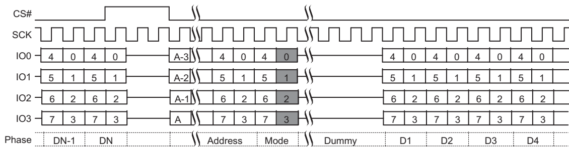
Figure 82. Continuous Quad I/O Read Command Sequence (EBh or ECh) [58, 59]
