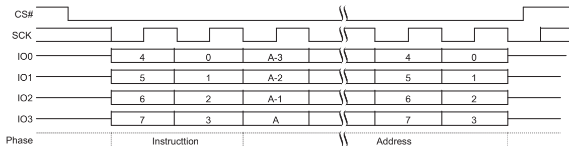
Figure 91. Sector Erase (SE D8h or 4SE DCh) QPI Mode Command Sequence [69]
