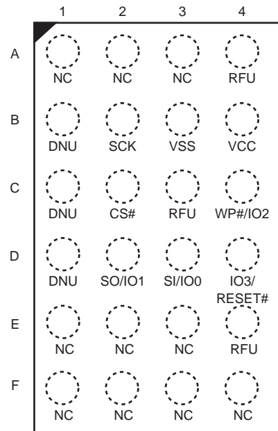
Figure 44. 24-Ball BGA, 4x6 Ball Footprint (FAC024), Top View [36, 37]
