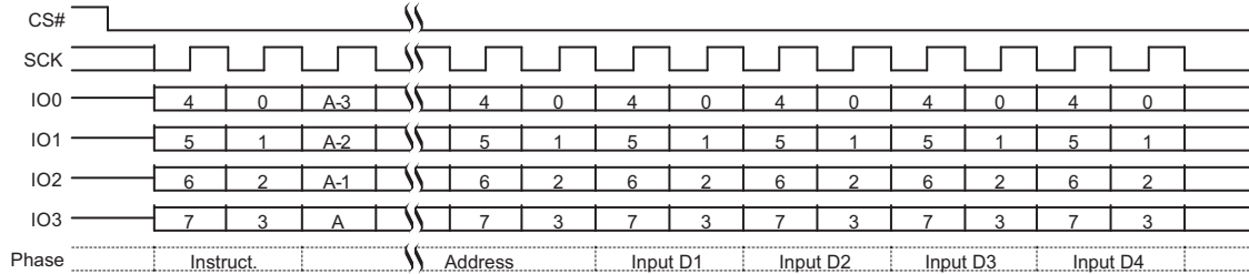
Figure 87. Page Program (PP 02h or 4PP 12h) QPI Mode Command Sequence [65]
