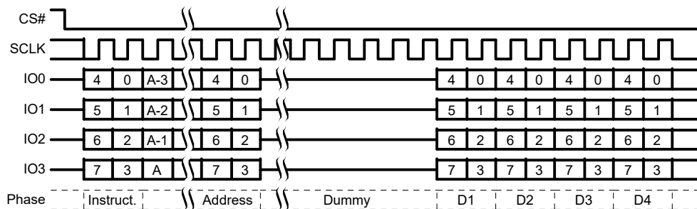
Figure 68. ECCRD (19h) or 4EECRD (18h), QPI Mode, Command Sequence [48, 49]
