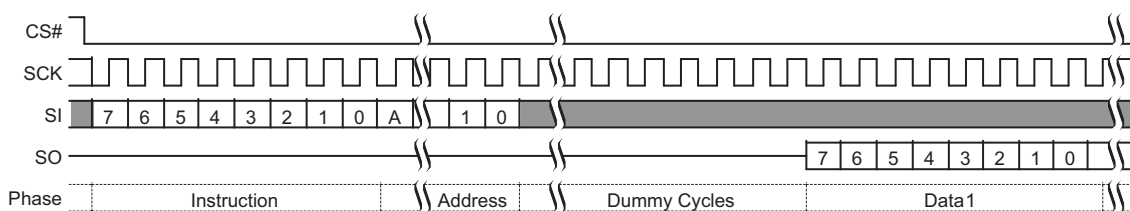
Figure 77. Fast Read (FAST_READ) Command Sequence (3-Byte Address, 0Bh [CR2V[7]=0]) [52]
