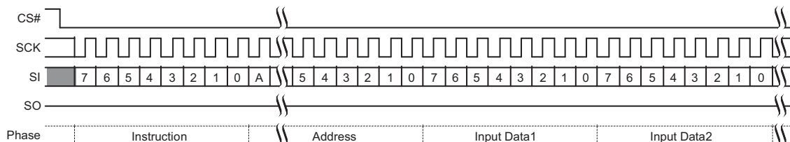
Figure 86. Page Program (PP 02h or 4PP 12h) Command Sequence [64]
