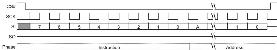
Figure 94. EES Command Sequence [70]
