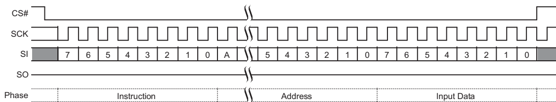
Figure 105. DYBWR Command Sequence [73, 74]
