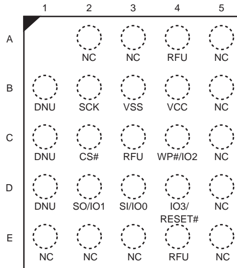
Figure 42. 24-Ball BGA, 5x5 Ball Footprint (FAB024), Top View [34, 35]
