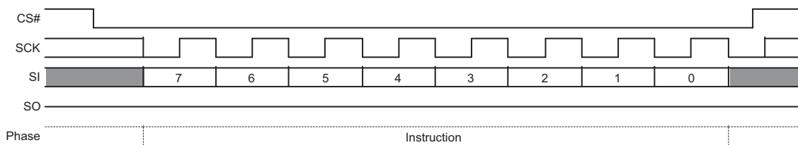
Figure 63. Write Disable (WRDI) Command Sequence
