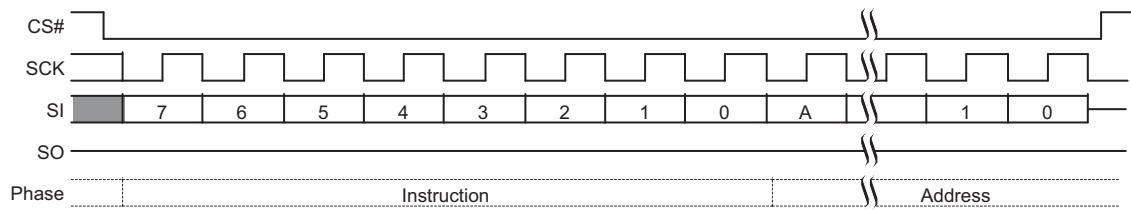
Figure 90. Sector Erase (SE D8h or 4SE DCh) Command Sequence [68]
