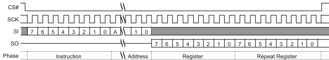
Figure 103. DYBRD Command Sequence [71, 72]
