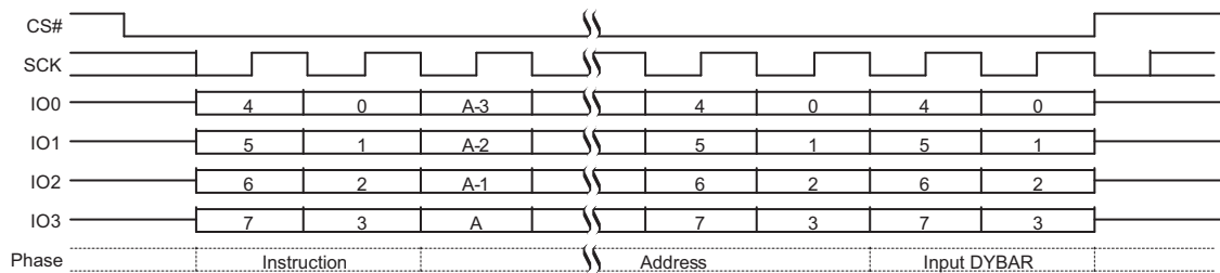
Figure 106. DYBWR QPI Mode Command Sequence [73, 74]
