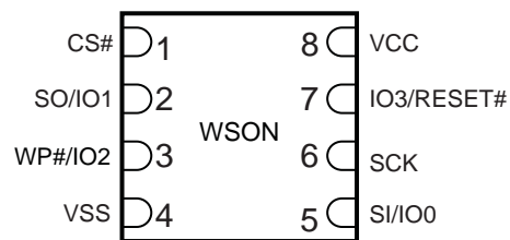
Figure 38. 8-Connector Package (WSON 6x5), Top View [33]
