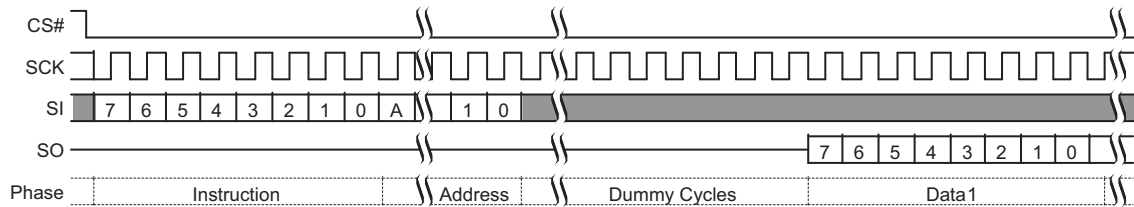
Figure 73. Read Any Register Read Command Sequence [50]
