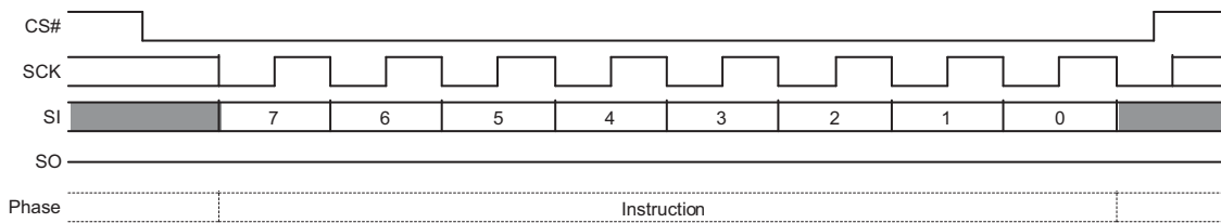
Figure 97. Program or Erase Suspend Command Sequence
