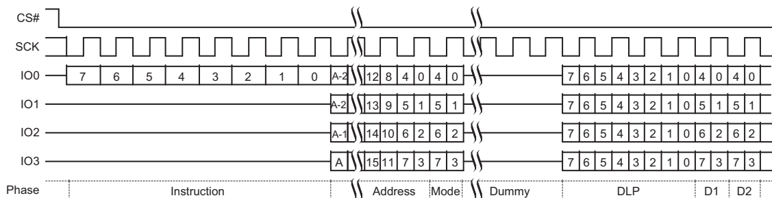
Figure 83. DDR Quad I/O Read Initial Access (EDh or EEh) [60, 61]
