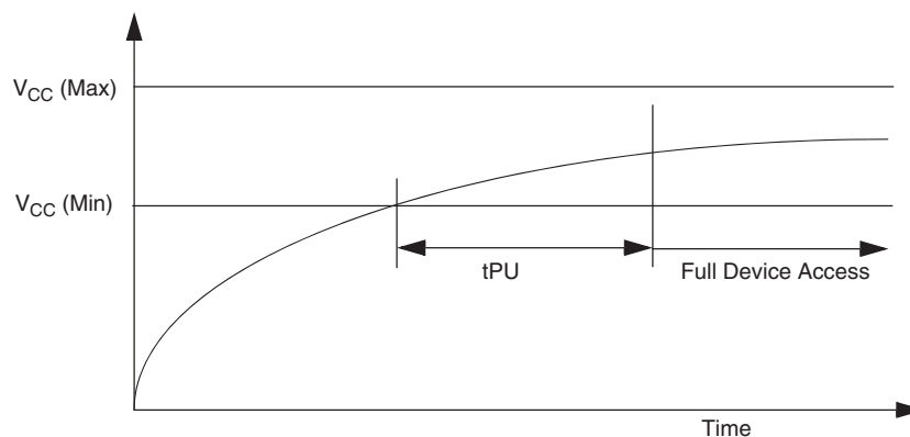
Figure 18. Power-Up
