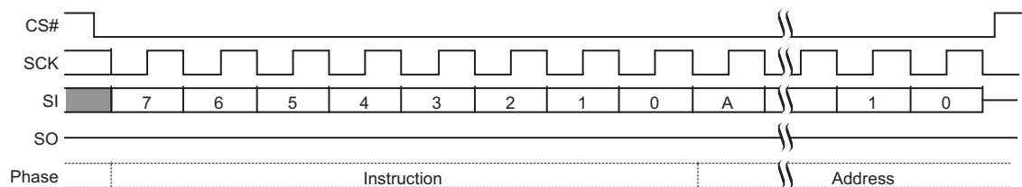
Figure 108. PPBP Command Sequence [77, 78]
