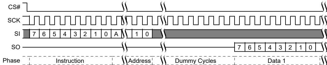
Figure 67. ECC Status Register Read Command Sequence [48, 49]
