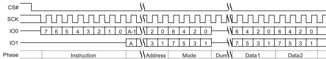
Figure 78. Dual I/O Read Command Sequence (BBh) [53, 54, 55]
