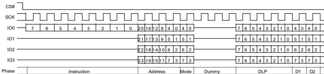
Figure 95. Continuous DDR Quad I/O Read Subsequent Access (3-Byte Address, HPLC=11b)
