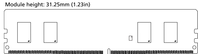
Figure 1: 288-Pin UDIMM (R/C C)
