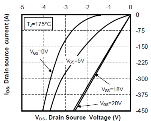
Figure 13 • 3 rd Quadrant Characteristics, T J = 175 °C
