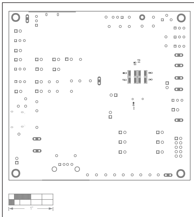
MAX77958-2S/3S EV Kit PCB Layout—Silkscreen Bottom
