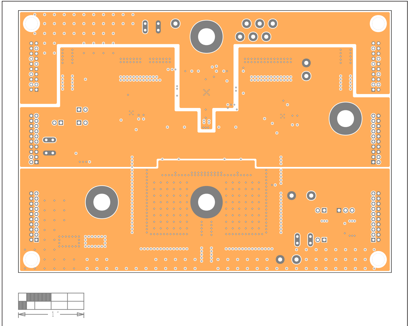
EV Kit PCB Layout—Internal Layer 5
