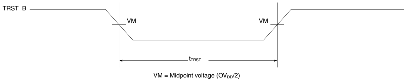
Figure 62. TRST_B timing diagram
