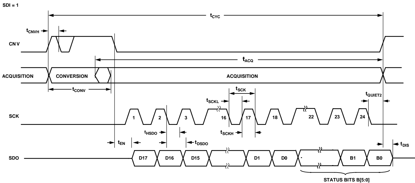
Figure 54. \overline{CS} Mode, 3-Wire Without Busy Indicator Serial Interface Timing Diagram Including Status Bits (SDI High)
