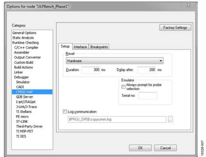
Figure 11. CMSIS DAP—Setup Tab
