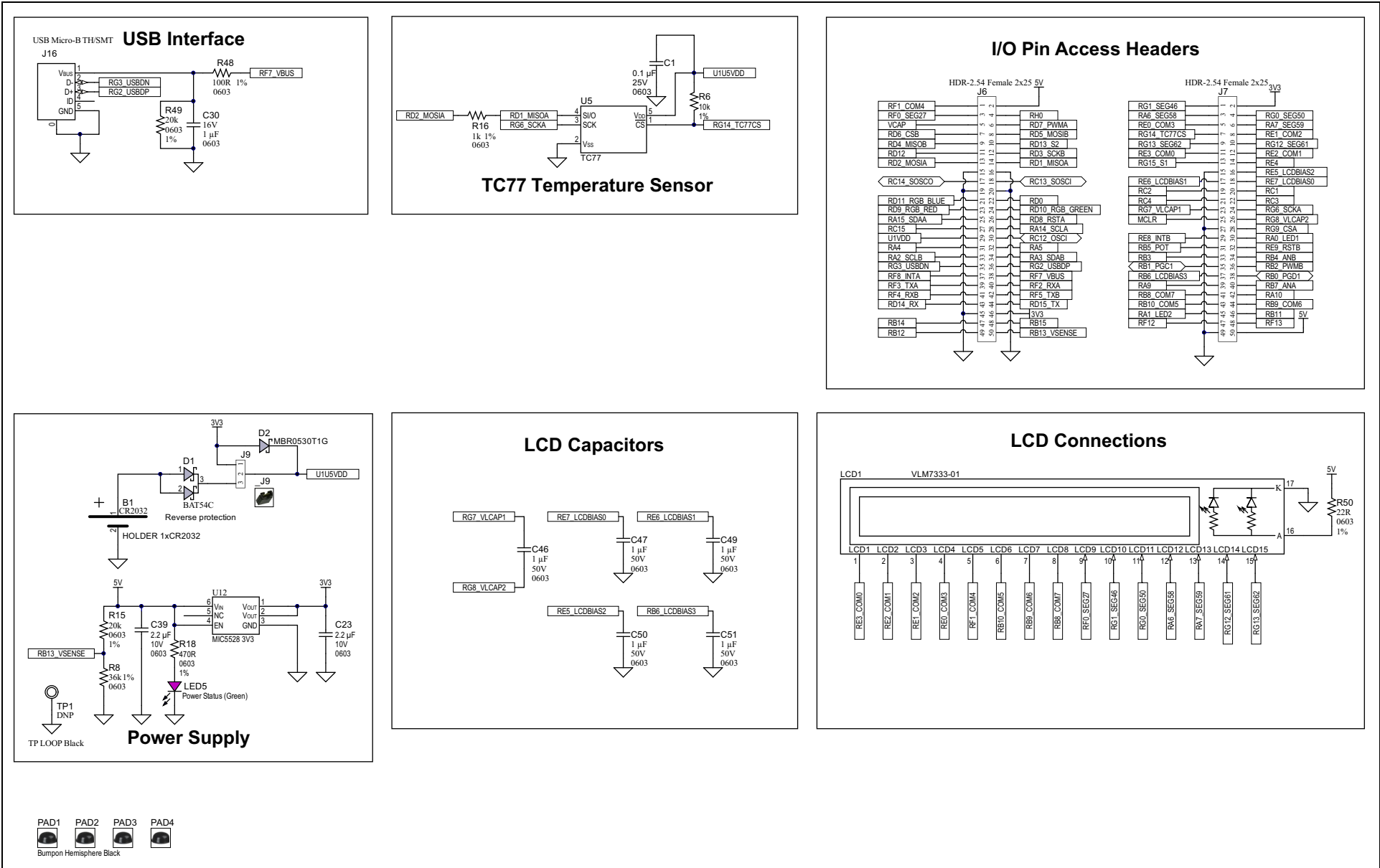
FIGURE 4: I/O ACCESS SCHEMATIC
