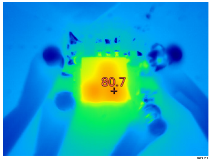
Figure 21. Thermal Image of LTM8083 Running from 24V Input and 36V Output with 1A Load at 25°C Ambient without Airflow or Heat Sink
