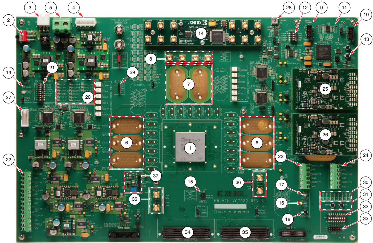
Figure 1-2: VC7222 Board Features. Callouts Listed in Table 1-1
