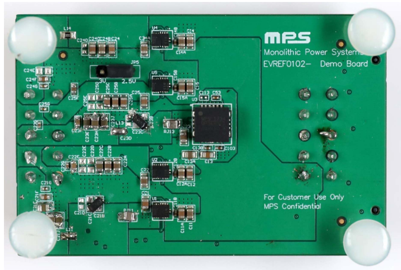
Figure 1-6: MPS Analog Power Module
