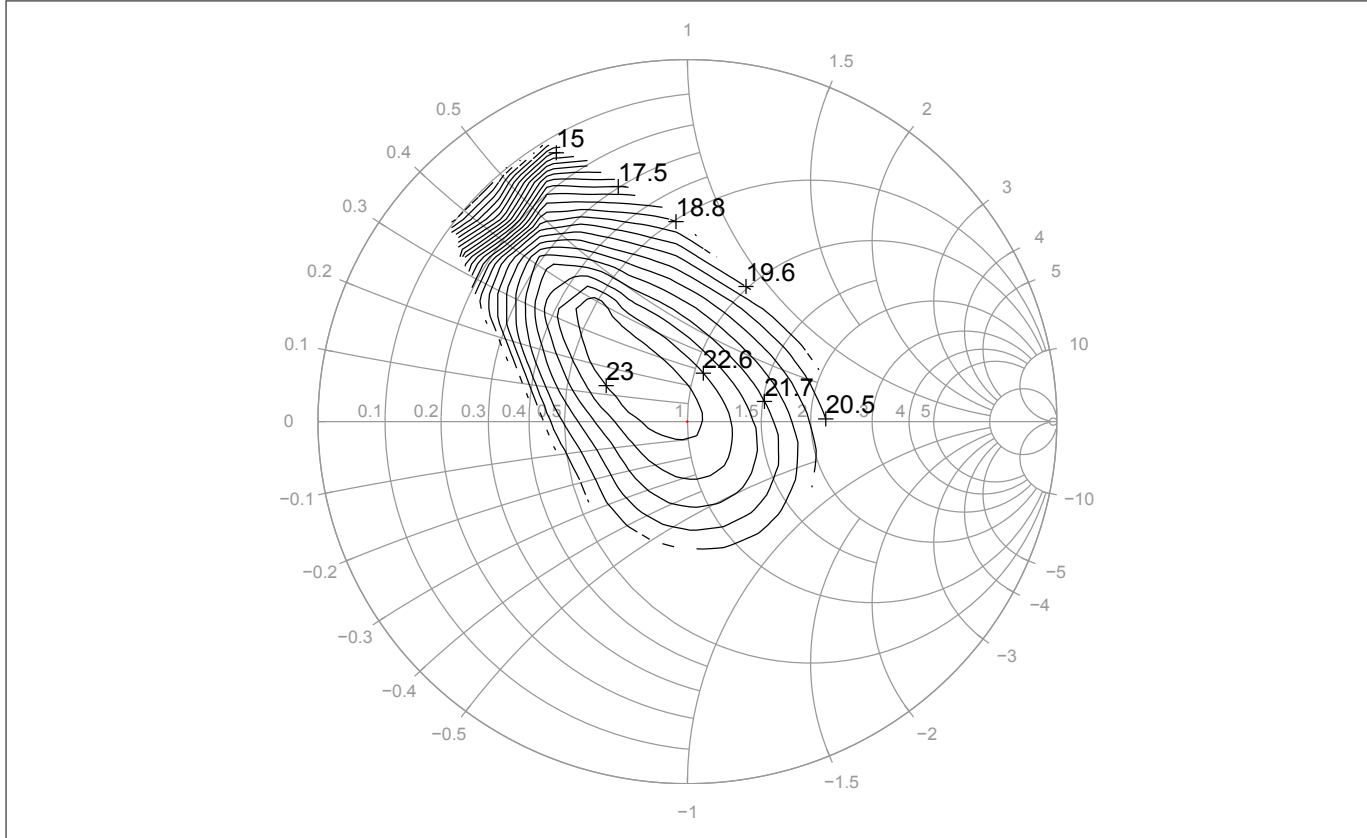
Figure 17 Load pull contour OP_{1dB} [dBm], V_{CE} = 5 V, I_C = 90 mA, f = 900 MHz
