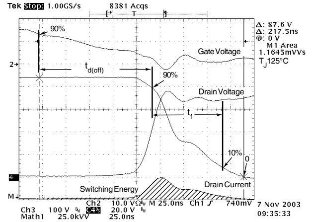
Figure 19, Turn-on Switching Waveforms and Definitions
