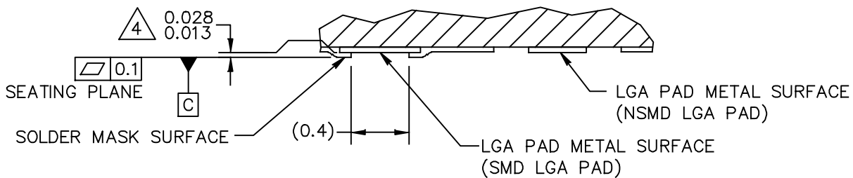
VIEW D-D (BOTTOM VIEW)
