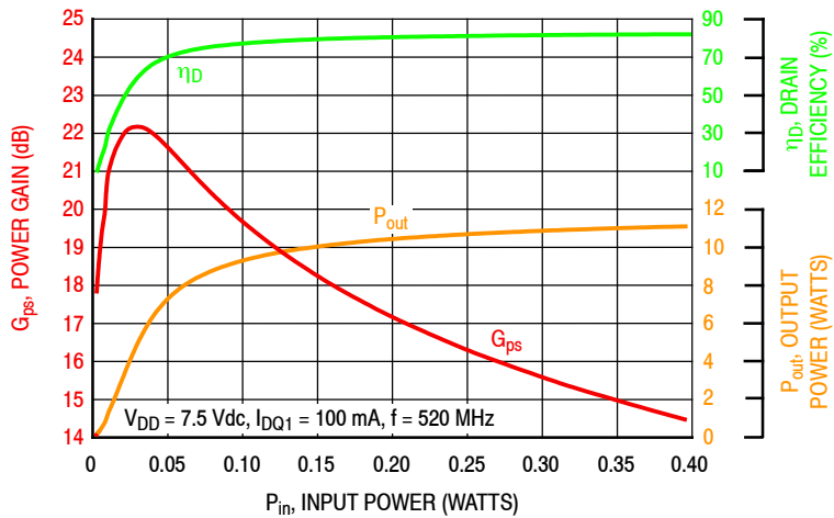
Figure 11. Power Gain, Drain Efficiency and Output Power versus Input Power
