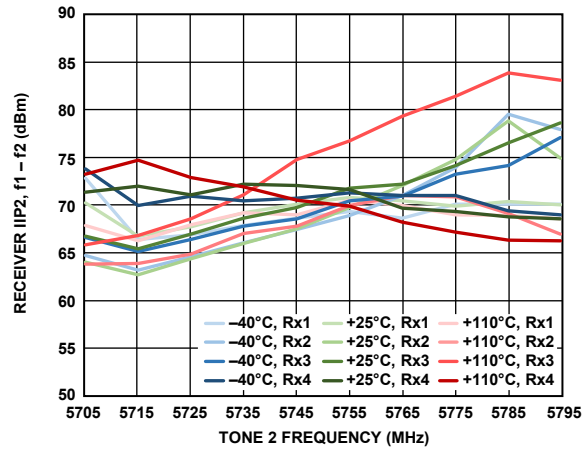
Figure 550. Receiver IIP2, f_1 - f_2 vs. Tone 2 Frequency, Both Tones at -11 dBFS, f_1 = f_2 + 2 MHz
