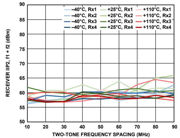
Figure 551. Receiver IIP2, f_1 + f_2 vs. Two-Tone Frequency Spacing, Both Tones at -11 dBFS, f_2 = 2 MHz
