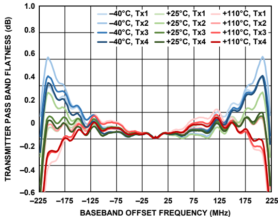
Figure 515. Transmitter Pass Band Flatness vs. Baseband Offset Frequency
