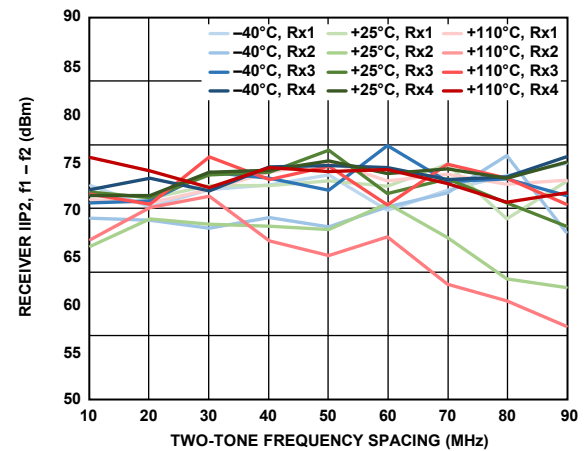
Figure 552. Receiver IIP2, f_1 - f_2 vs. Two-Tone Frequency Spacing, Both Tones at -11 dBFS, f_2 = 2 MHz
