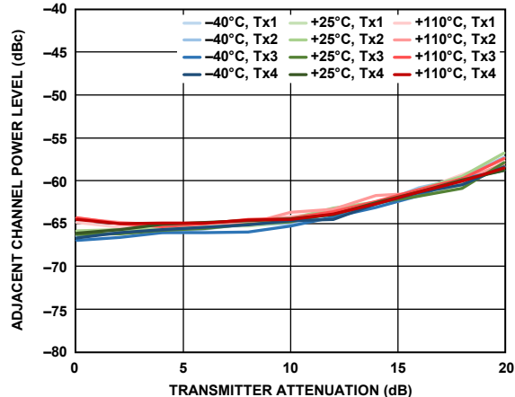
Figure 516. Adjacent Channel Power Level vs. Transmitter Attenuation, -10 MHz Baseband Offset, 20 MHz LTE, PAR = 12 dB
