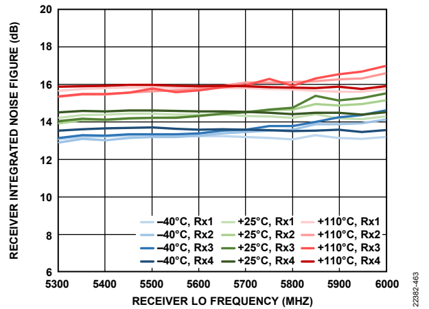
Figure 534. Receiver Integrated Noise Figure vs. Receiver LO Frequency, 200 MHz Bandwidth, Sample Rate = 245.76 MSPS, Integration Bandwidth = 500 kHz to 100 MHz
