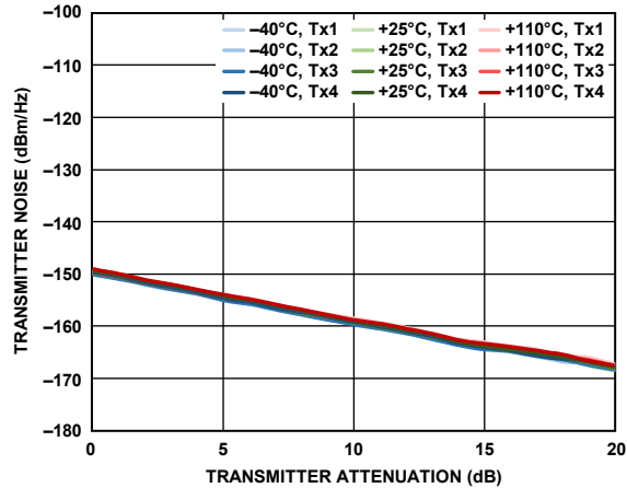
Figure 514. Transmitter Noise vs. Transmitter Attenuation, 10 MHz Offset Frequency
