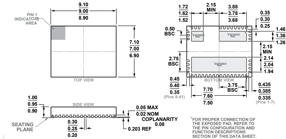
Figure 79. 41-Lead Lead Frame Chip Scale Package [LFCSP] 9 mm x 7 mm Body and 0.95 mm Package Height (CP-41-1) Dimensions shown in millimeters
