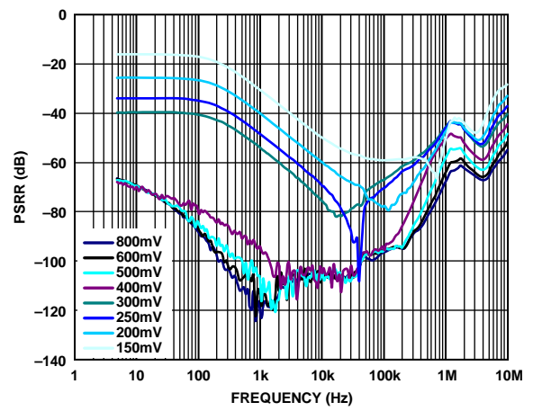
Figure 22. Power Supply Rejection Ratio (PSRR) vs. Frequency at Various Headroom Voltages, V_{OUT} = 3.3\text{ V} , 400 mA Load
