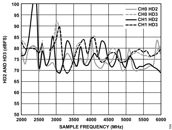
Figure 36. HD2 and HD3 vs. Sample Frequency ( f_s ), f_{IN} = 450 MHz, A_{IN} = -1 dBFS, f_s = 2 GSps to 6 GSps
