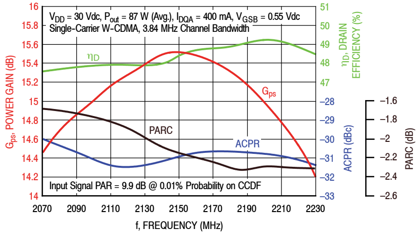
Figure 3. Single-Carrier Output Peak-to-Average Ratio Compression (PARC) Broadband Performance @ P_{out} = 87 Watts Avg.
