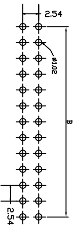
PCB LAYOUT
