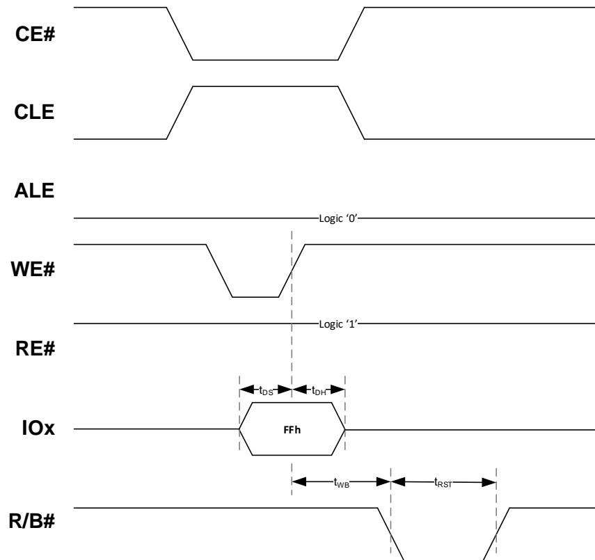
Figure 8: RESET Operation
