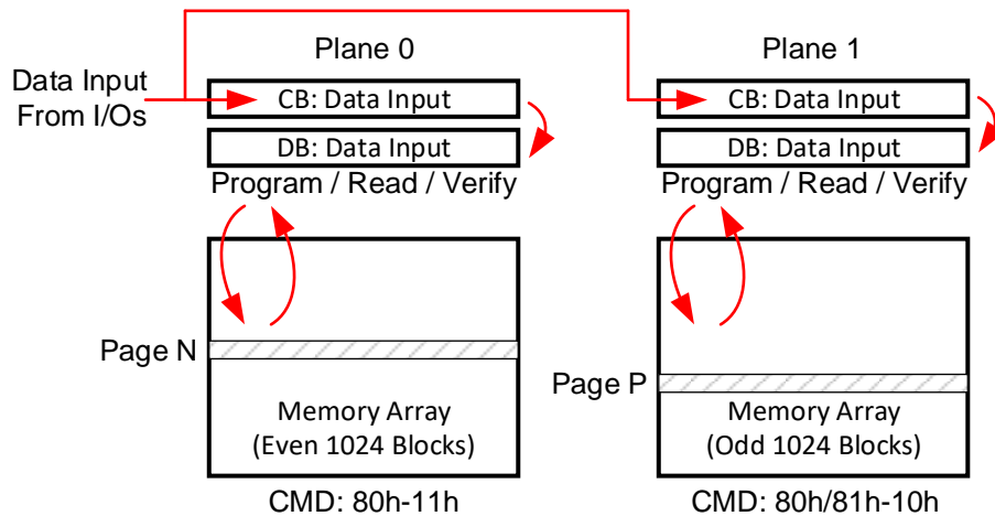
Figure 29: Program Page MP Operation Overview
