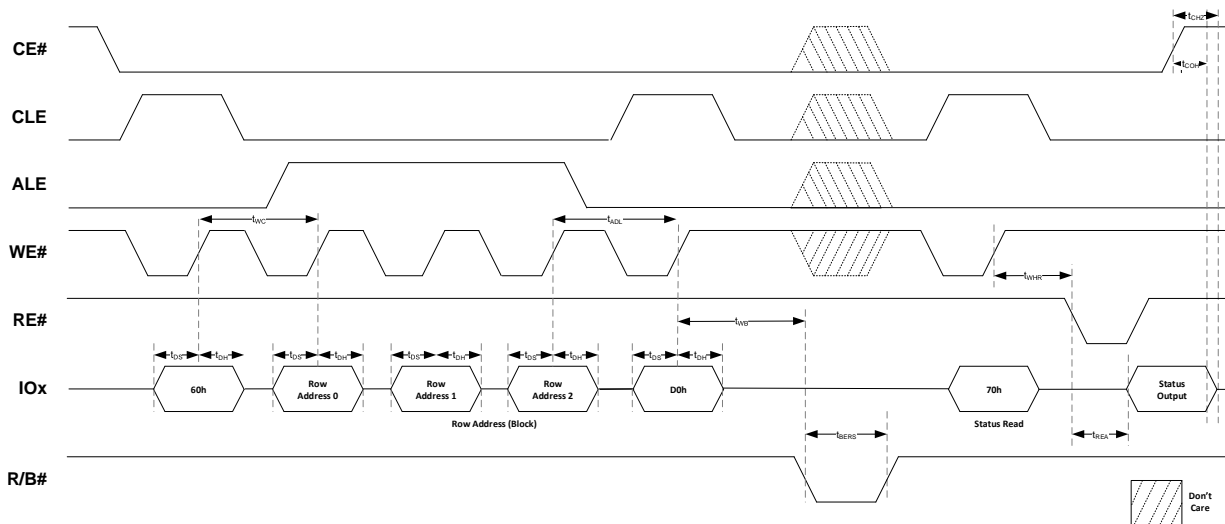
Figure 25: Erase Block Operation
