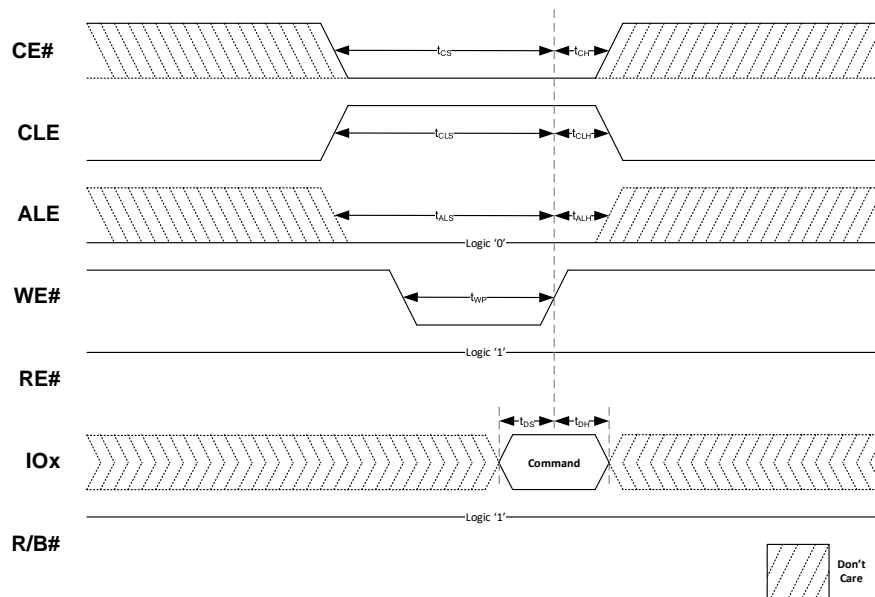
Figure 4: Command Latch Cycle
