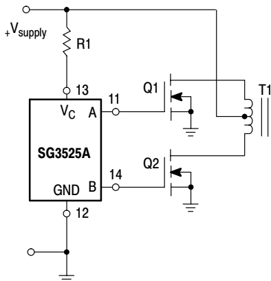
Figure 10. Single-Ended Supply
