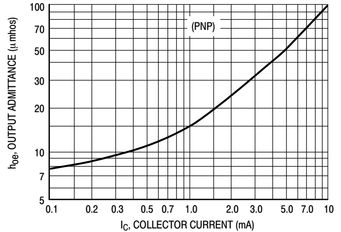
Figure 27. Output Admittance
